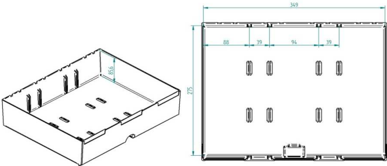
Drawer BIG
